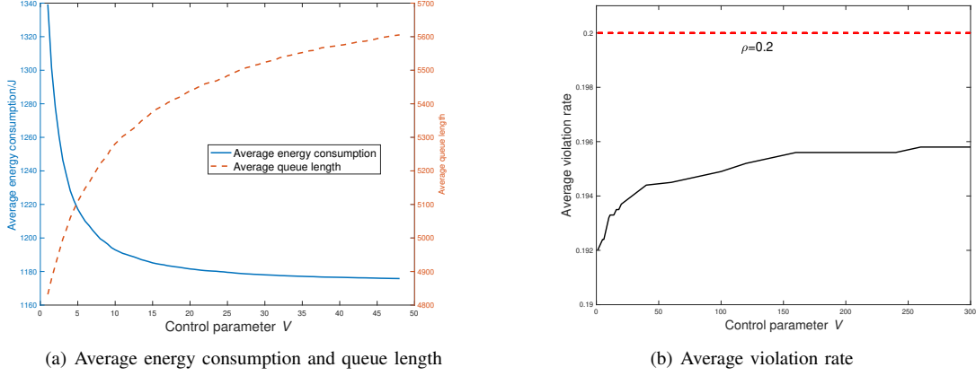
Fig. 2: Impact of V on average energy consumption, queue length and violation rate
