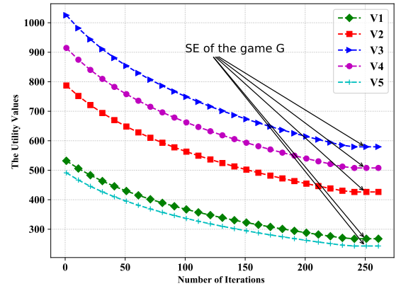
Fig. 1. The utility values of four vehicles before reaching SE of the game
