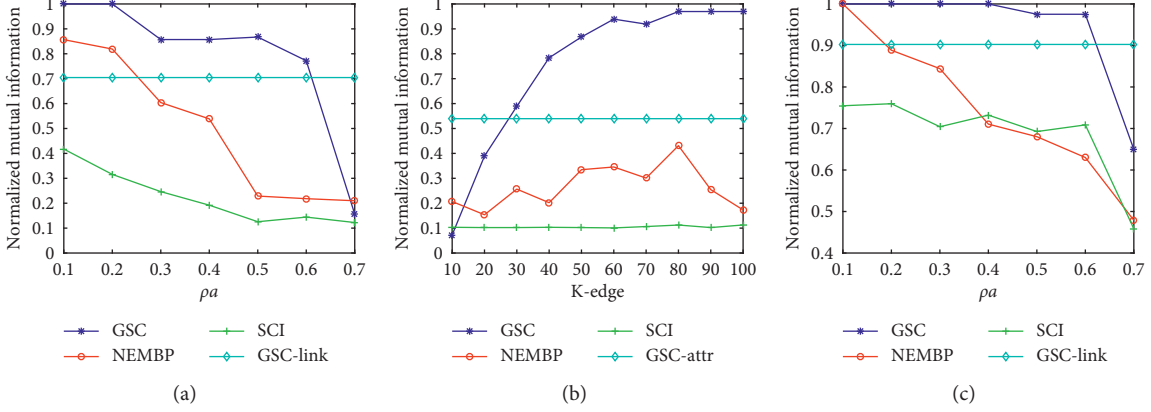
FIGURE 7: The value of NMI of four methods: (a) on Synthetic 108 with the change of \rho_a from 0.1 to 0.7, (b) on Synthetic 108 with the change of keystone links from 10 to 100, and (c) on Synthetic 100 with the change of \rho_a from 0.1 to 0.7.
