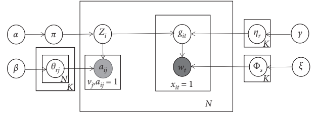
FIGURE 1: The graphical representation of model.
