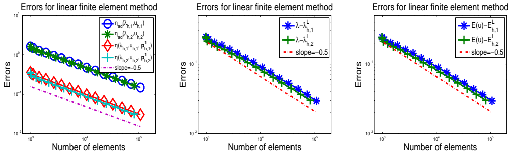
Figure 4: The errors for the L shape domain when the eigenvalue problem is solved by the linear finite element method. Here, \eta(\lambda_{h,1}, u_{h,1}, \mathbf{p}_{h,1}^1) denotes \eta(\lambda_{h,1}, u_{h,1}, \mathbf{p}_{h,1}^*) when the auxiliary problem is solved in \mathbf{W}_{h,1}^1 on the meshes which are generated by adaptive refinement with the a posteriori error estimator \eta_{ad}(\lambda_{h,1}, u_{h,1}) , \eta(\lambda_{h,2}, u_{h,2}, \mathbf{p}_{h,2}^1) denotes \eta(\lambda_{h,2}, u_{h,2}, \mathbf{p}_{h,2}^*) when the auxiliary problem is solved in \mathbf{W}_{h,2}^1 on the meshes which are generated by using the a posteriori error estimator \eta(\lambda_{h,2}, u_{h,2}, \mathbf{p}_{h,2}^1) .
