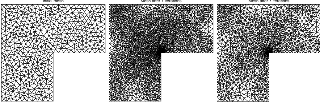
Figure 3: The initial mesh of L-shape domain (left), the mesh after 7 adaptive refinements using the a posteriori error estimator \eta_{ad}(\lambda_h, u_h) (middle) and the mesh after 7 adaptive refinements using the a posteriori error estimator \eta(\lambda_h, u_h, \mathbf{p}_h) (right).
