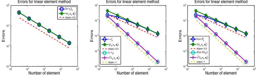
Figure 2: The errors for the unit square domain when the eigenvalue problem is solved by the linear finite element method, where \eta(\lambda_h, u_h, \mathbf{p}_h^1) denotes the a posteriori error estimator \eta(\lambda_h, u_h, \mathbf{p}_h^*) when the auxiliary problem is solved in \mathbf{W}_h^1 , \lambda_h^L denotes the asymptotically lower bound of the principal eigenvalue and E_h^L denotes the asymptotically lower bound of the ground state energy.
