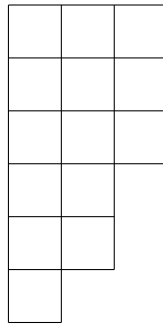
Figure 3.1: The shape of linked partition \{1, 2, 4\}\{2, 3\}\{3, 9\}\{5, 6\}\{6, 7\}\{8\} .
